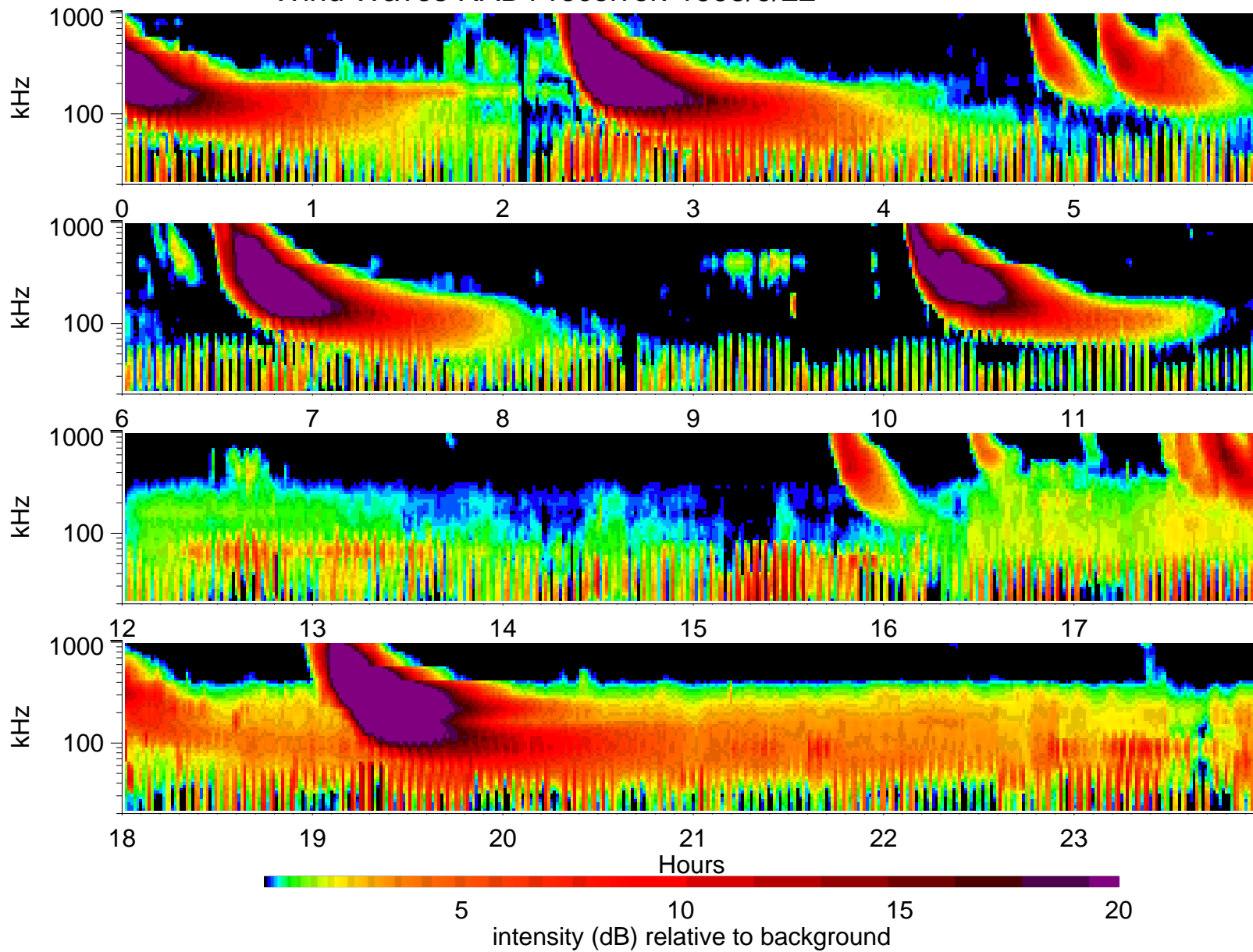
Wind Waves RAD1 receiver: 1995/9/22
