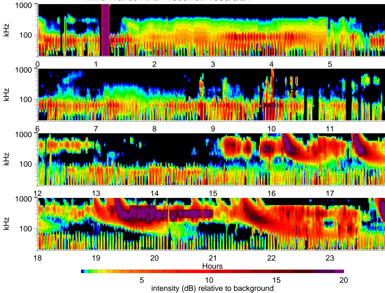
Wind Waves RAD1 receiver: 1995/9/21
