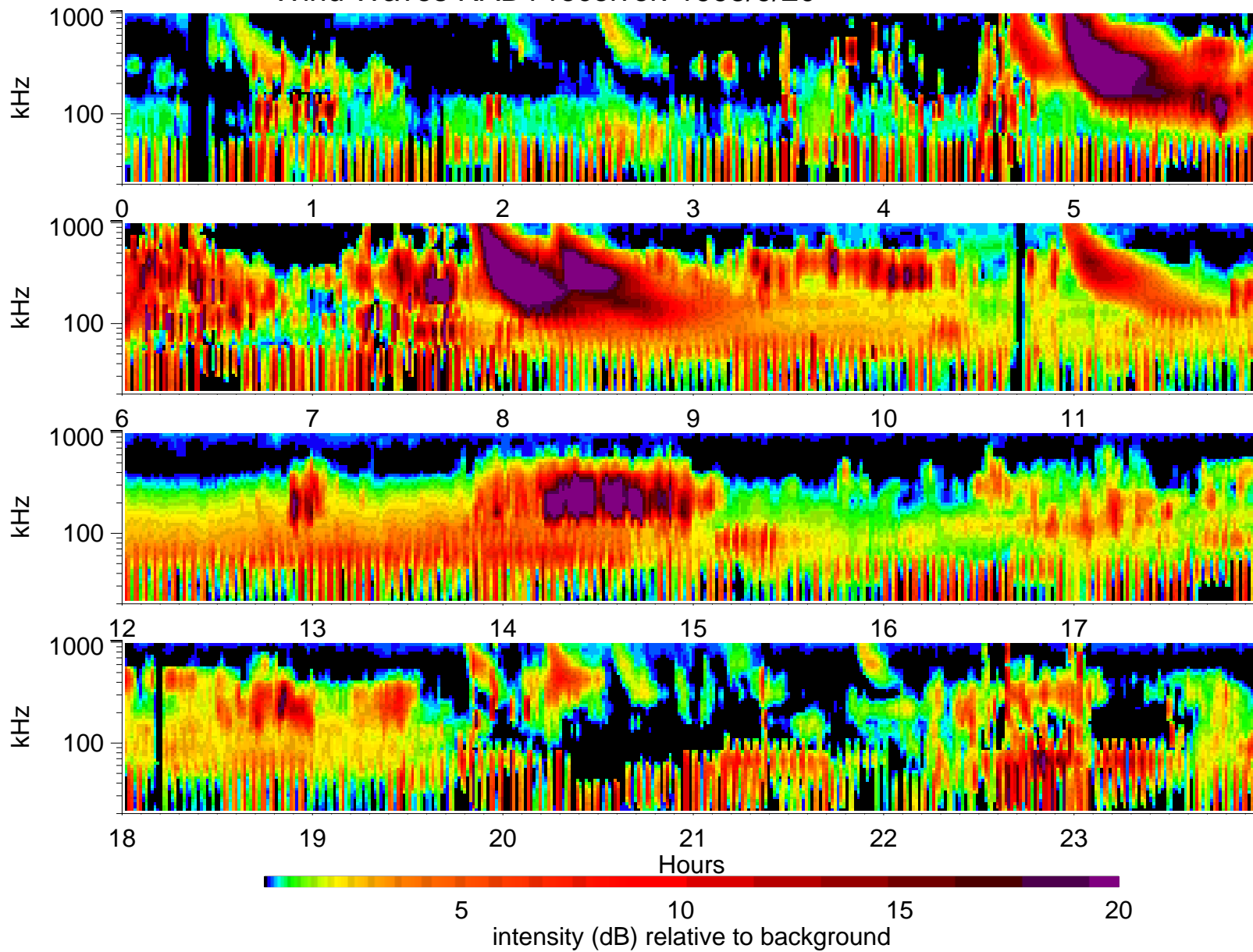
Wind Waves RAD1 receiver: 1995/9/20
