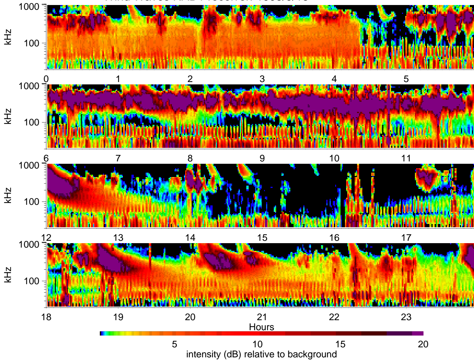
Wind Waves RAD1 receiver: 1995/9/18
