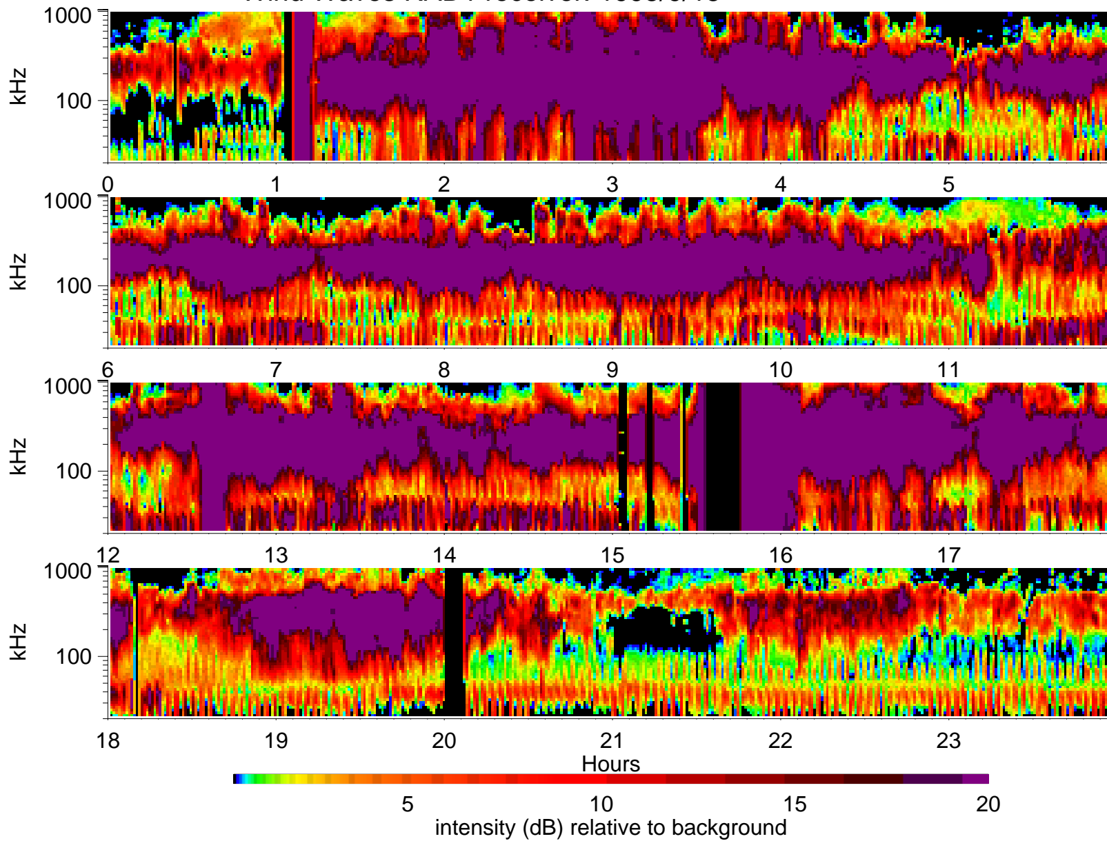
Wind Waves RAD1 receiver: 1995/9/15
