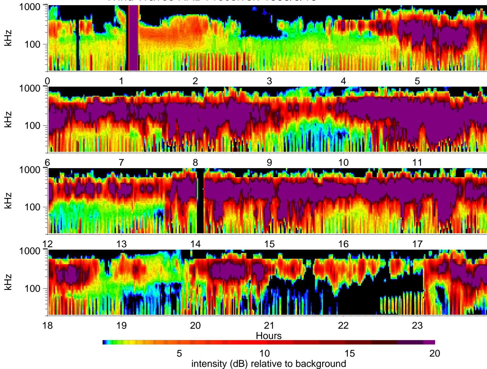
Wind Waves RAD1 receiver: 1995/9/13
