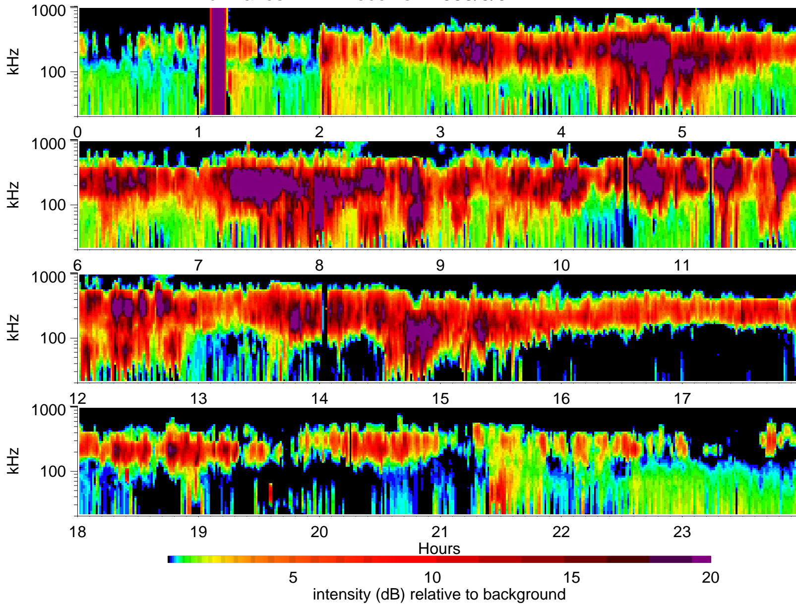
Wind Waves RAD1 receiver: 1995/9/9
