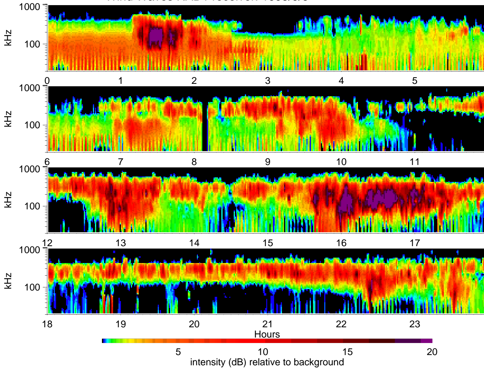
Wind Waves RAD1 receiver: 1995/9/6
