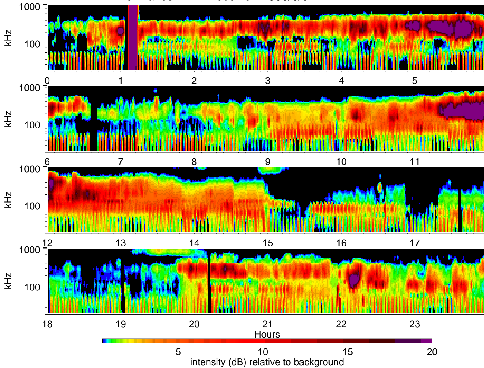
Wind Waves RAD1 receiver: 1995/9/5
