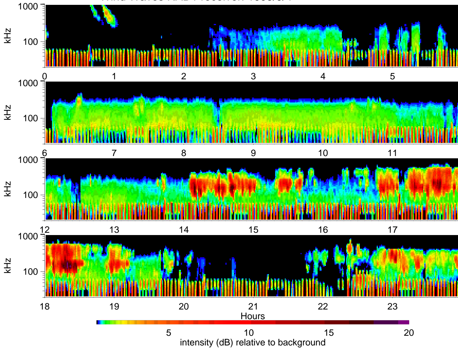
Wind Waves RAD1 receiver: 1995/9/4
