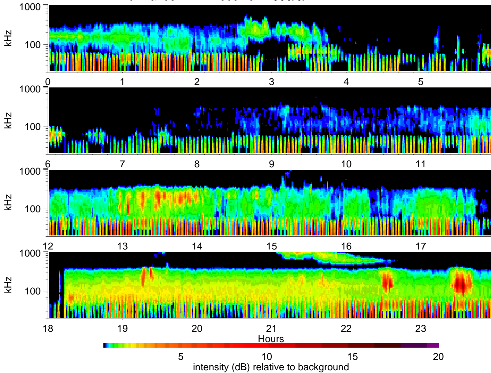
Wind Waves RAD1 receiver: 1995/9/2
