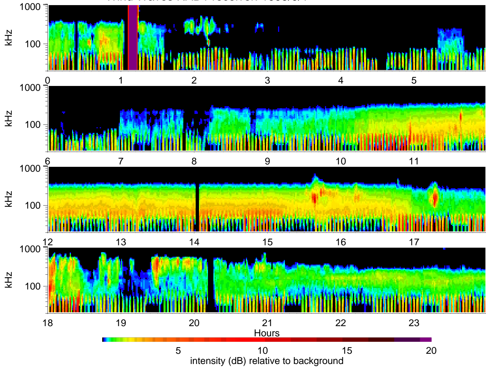
Wind Waves RAD1 receiver: 1995/9/1
