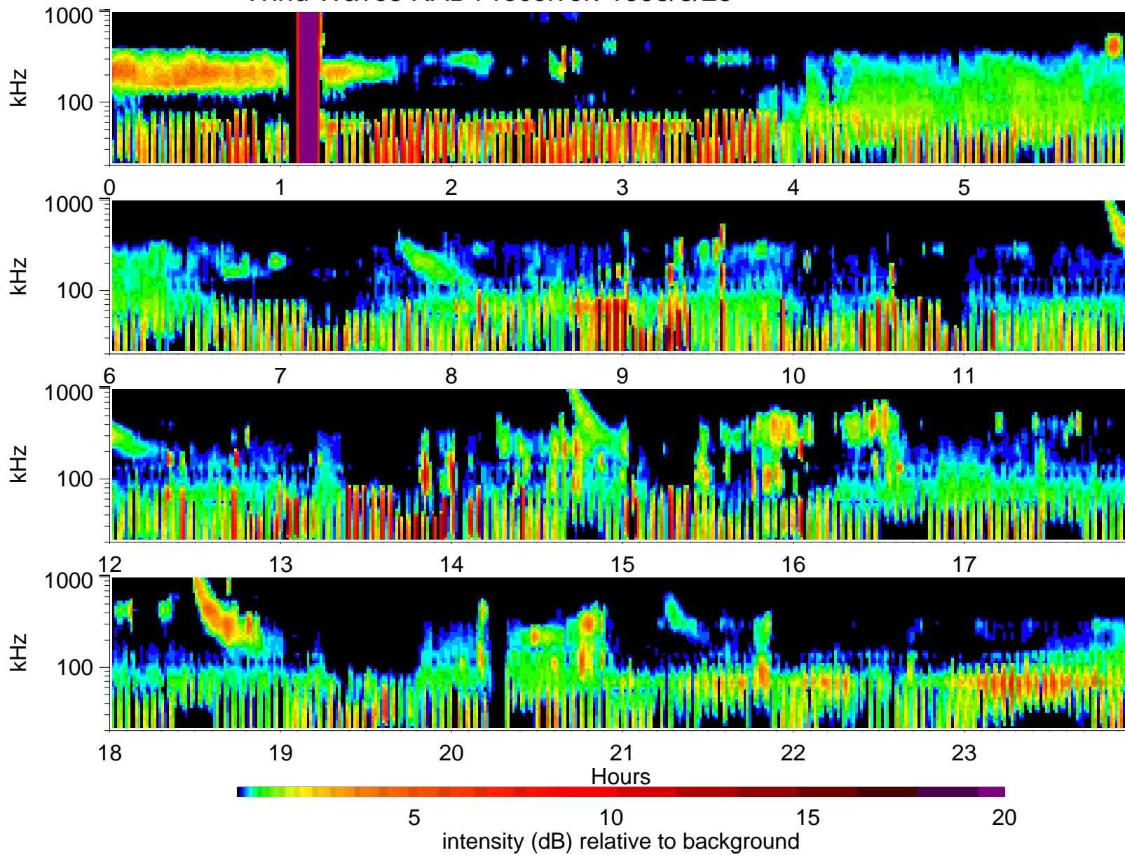
Wind Waves RAD1 receiver: 1995/8/28
