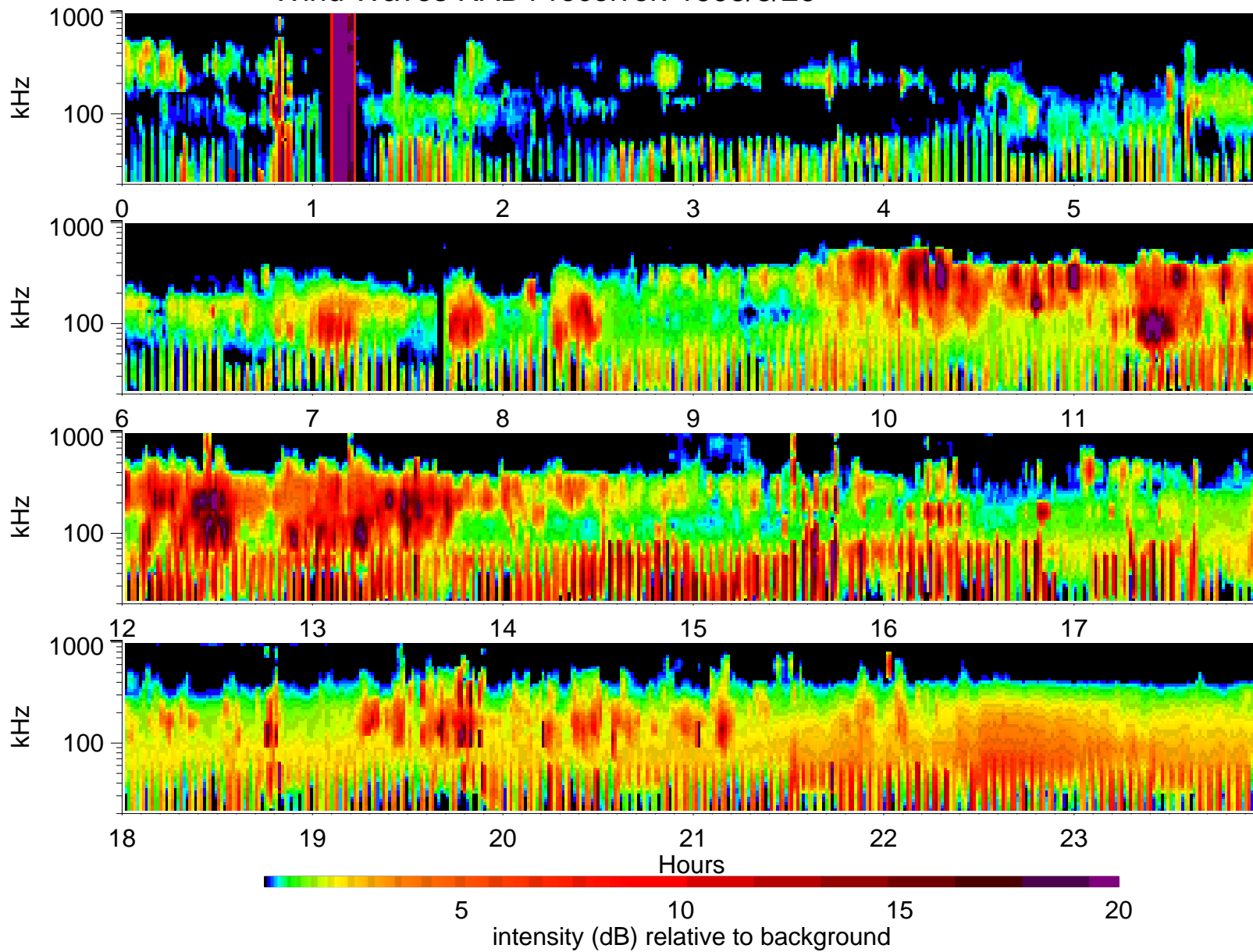
Wind Waves RAD1 receiver: 1995/8/26
