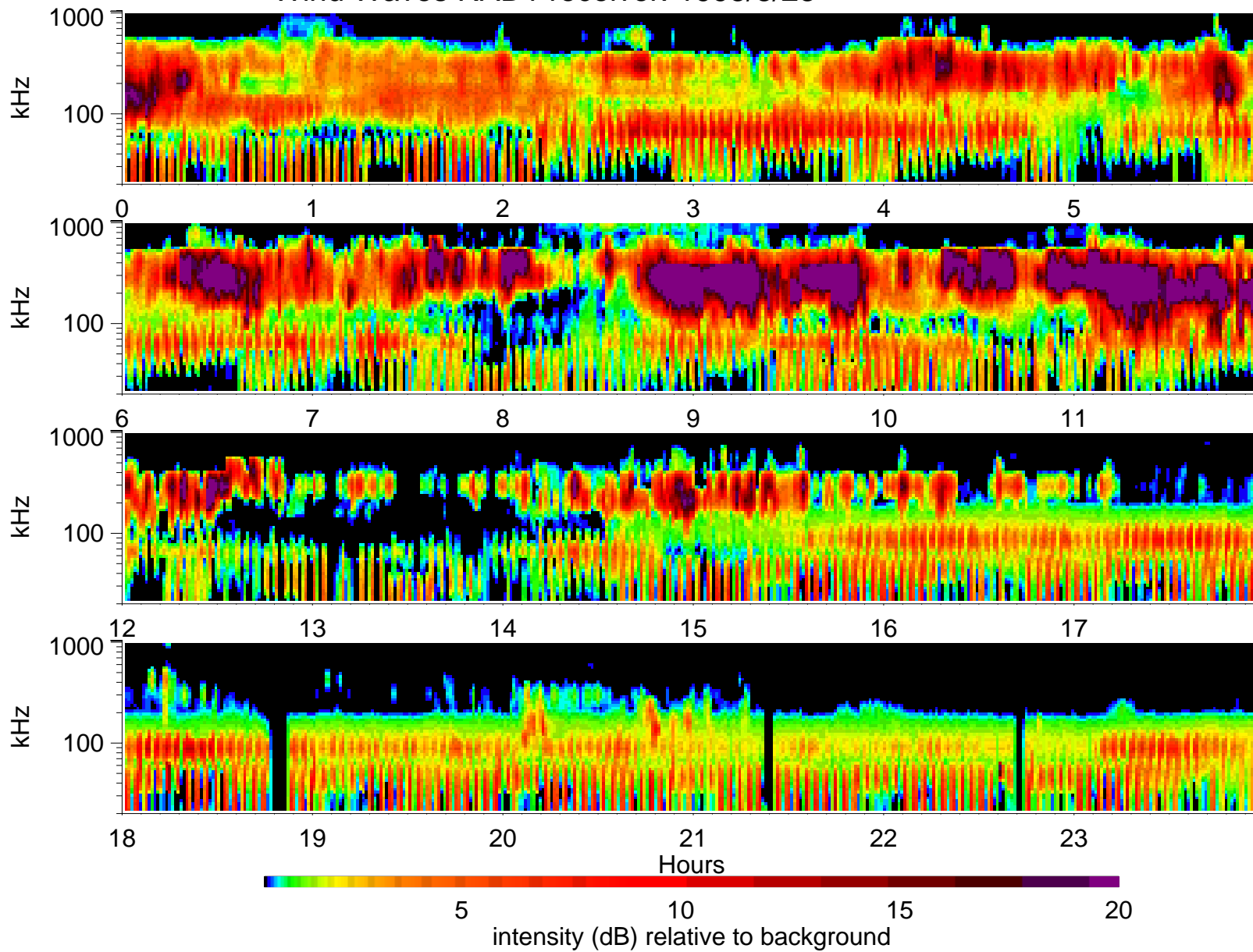
Wind Waves RAD1 receiver: 1995/8/23
