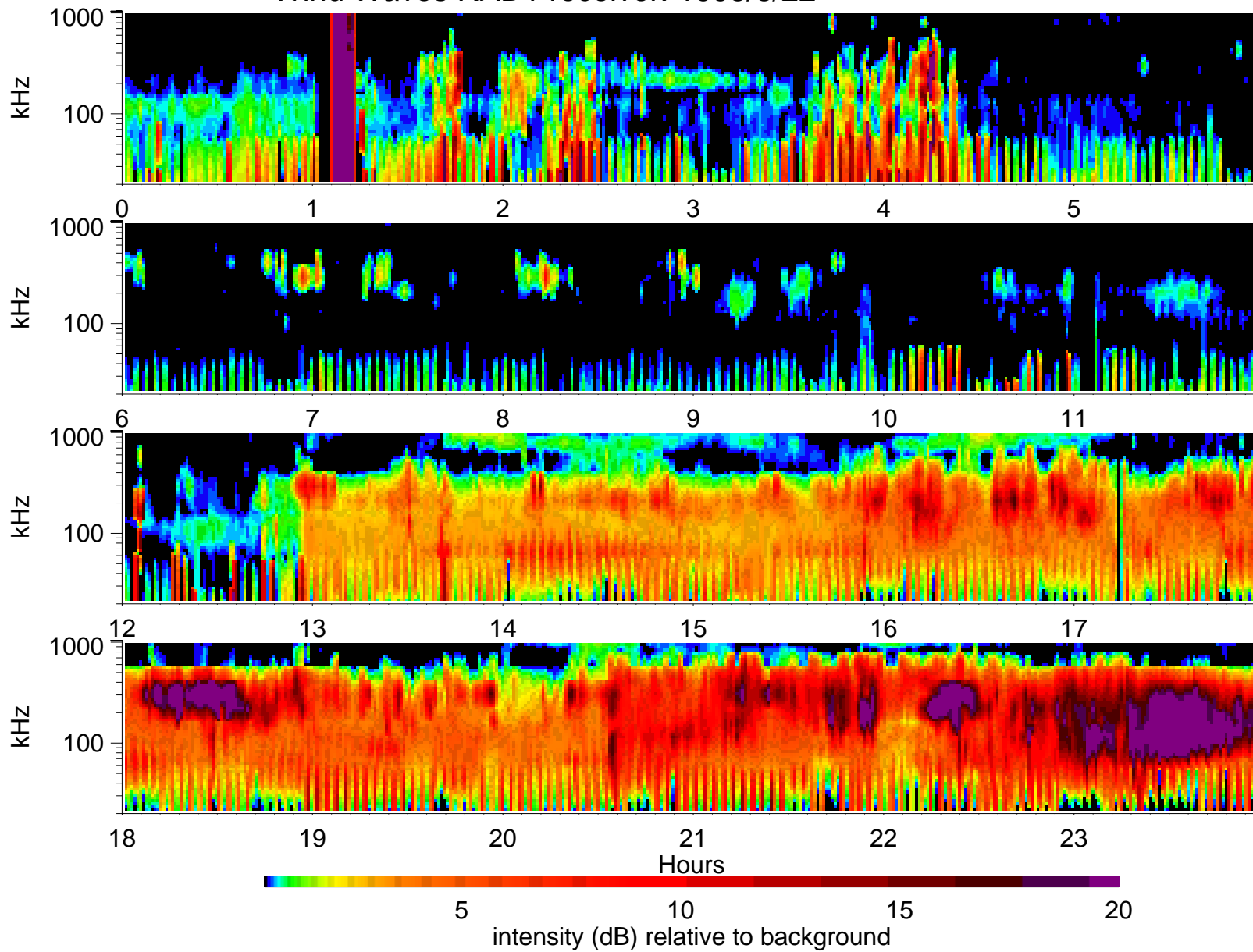
Wind Waves RAD1 receiver: 1995/8/22
