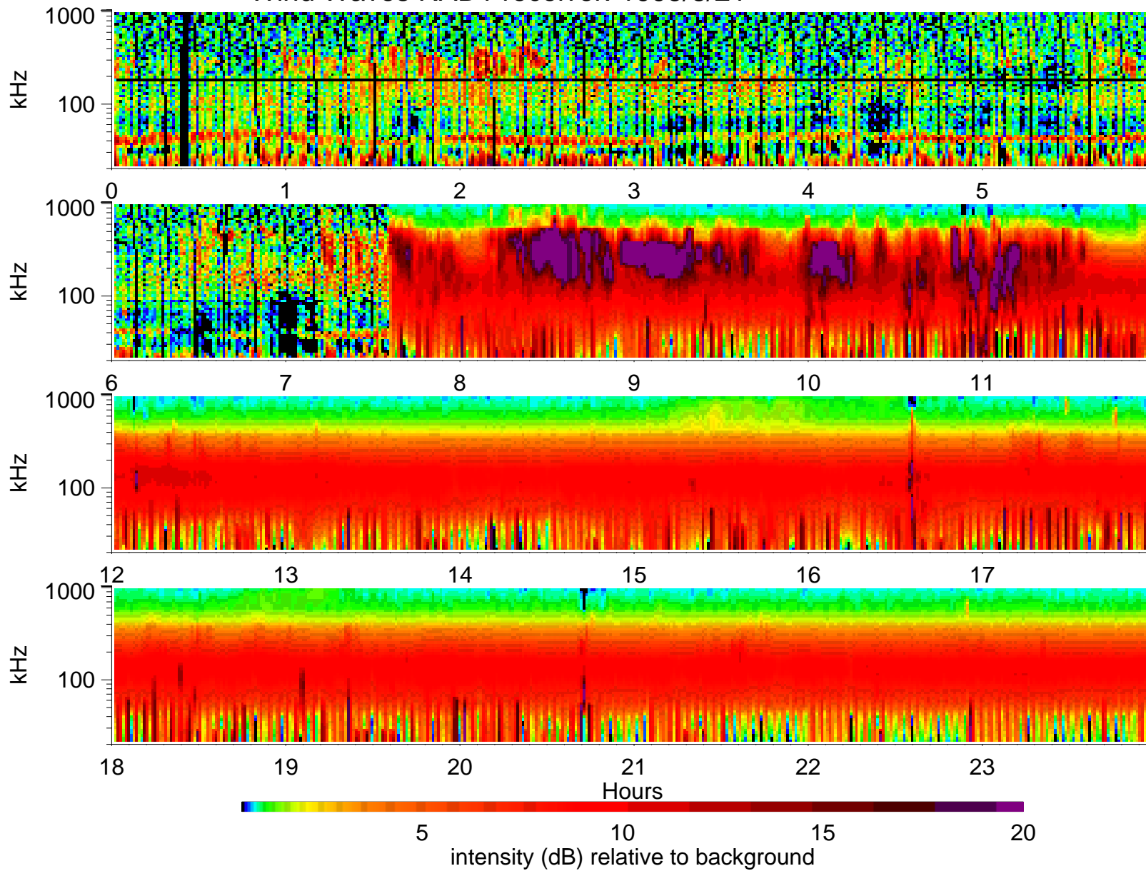
Wind Waves RAD1 receiver: 1995/8/21
