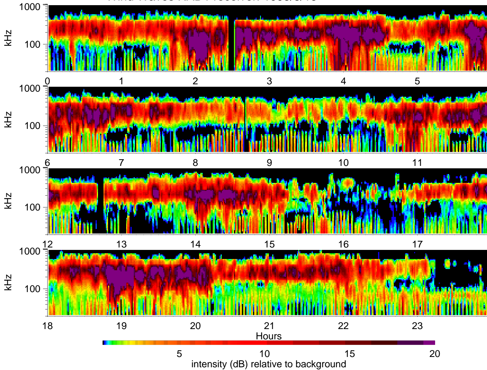
Wind Waves RAD1 receiver: 1995/8/15
