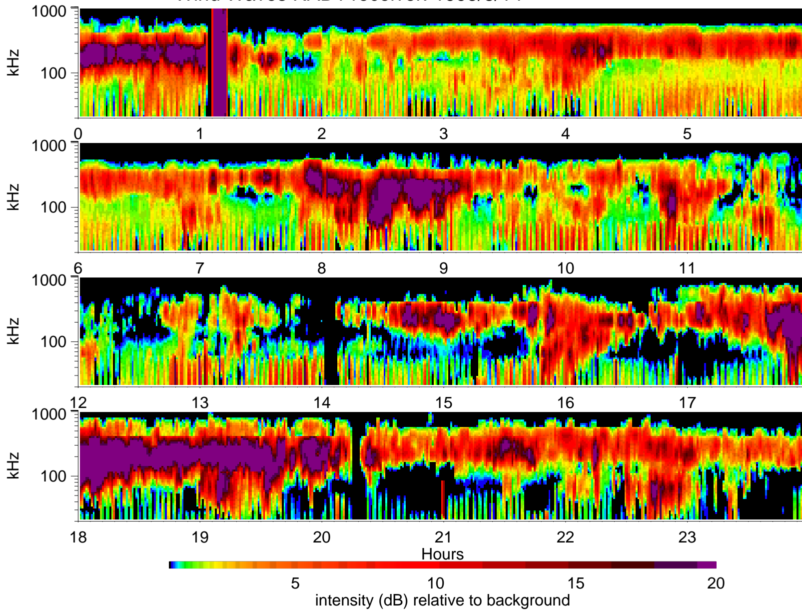
Wind Waves RAD1 receiver: 1995/8/14
