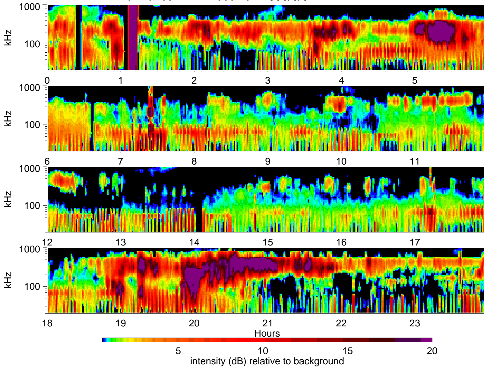
Wind Waves RAD1 receiver: 1995/8/8
