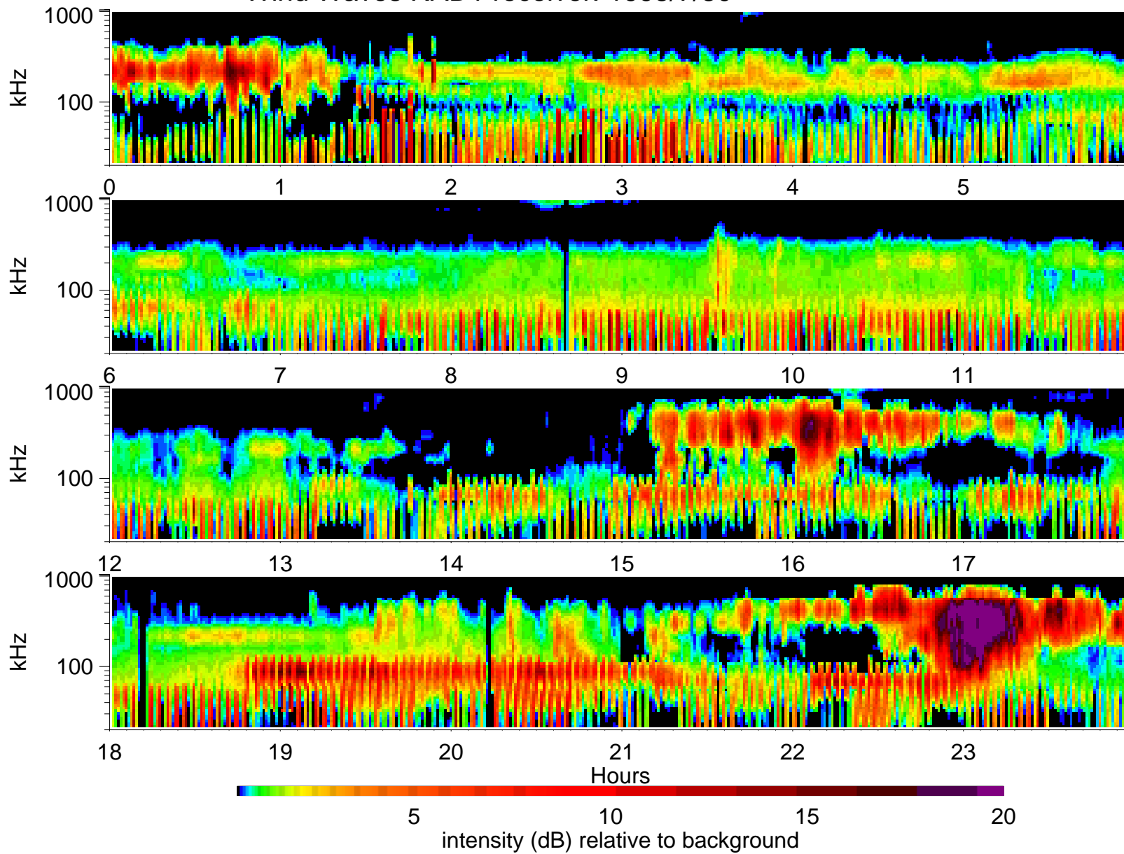
Wind Waves RAD1 receiver: 1995/7/30
