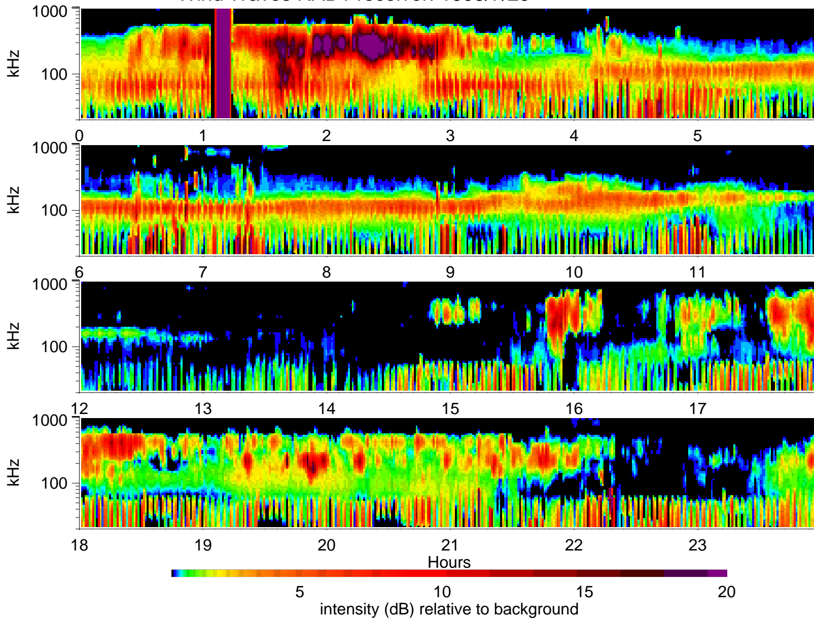
Wind Waves RAD1 receiver: 1995/7/29
