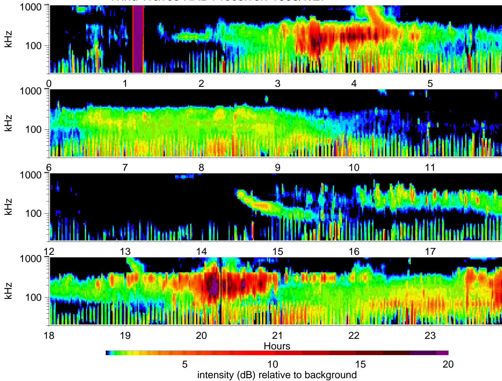
Wind Waves RAD1 receiver: 1995/7/27
