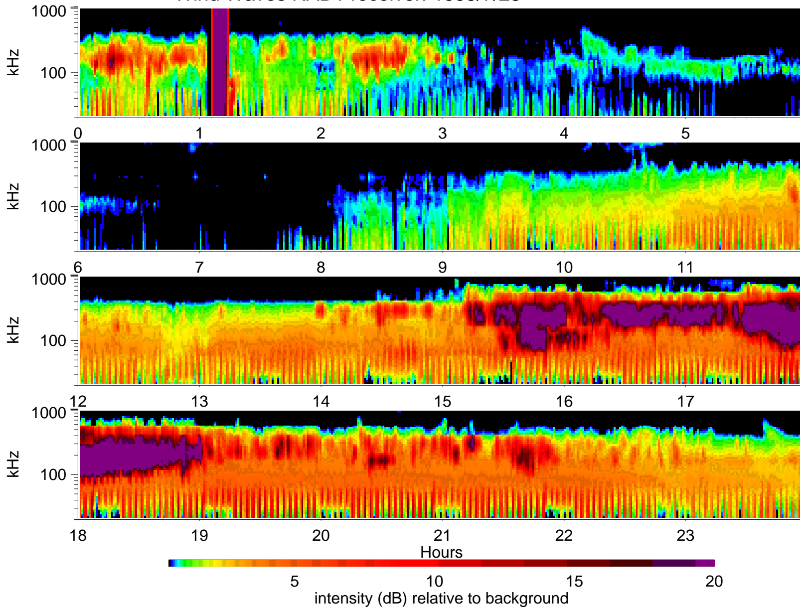
Wind Waves RAD1 receiver: 1995/7/23
