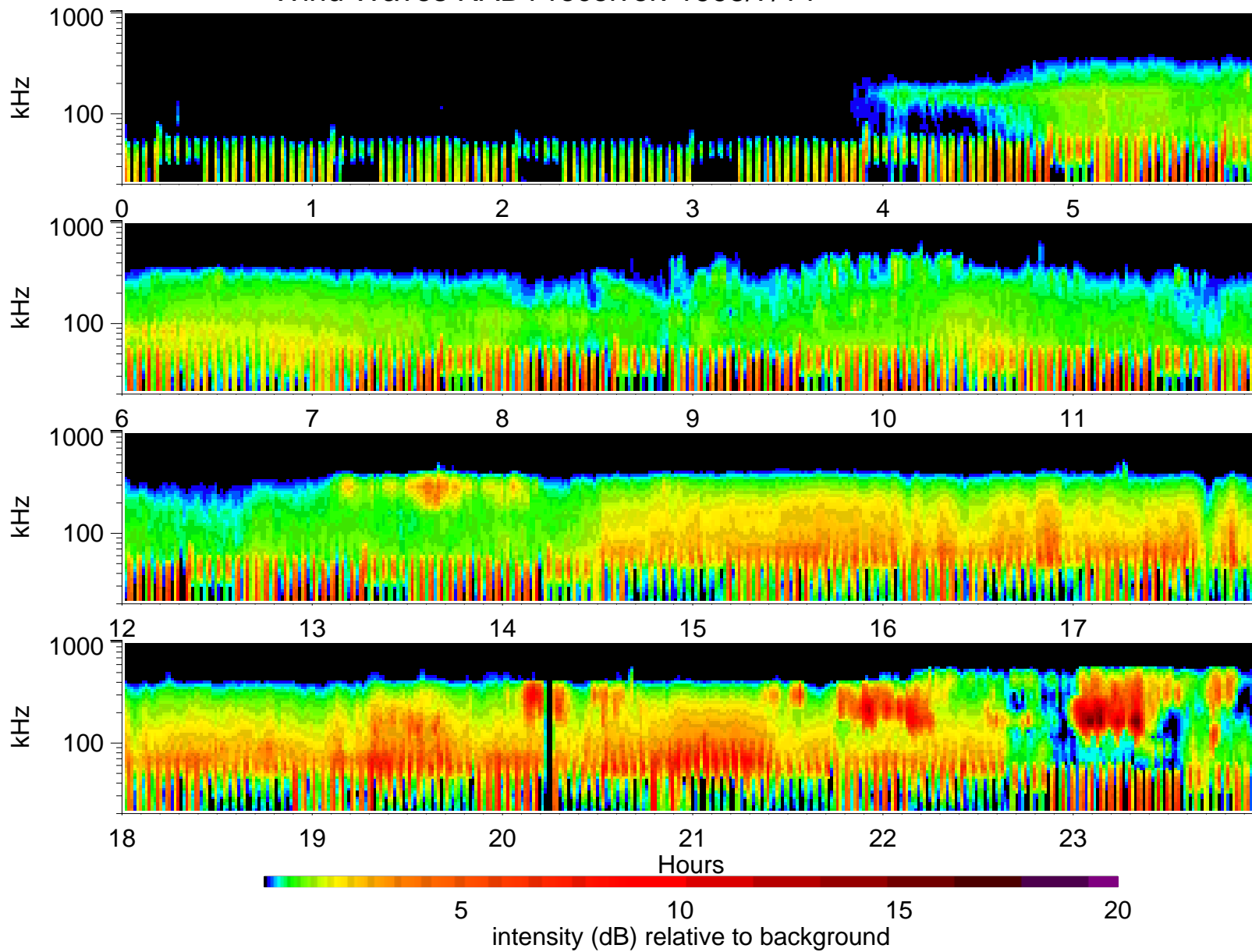
Wind Waves RAD1 receiver: 1995/7/14
