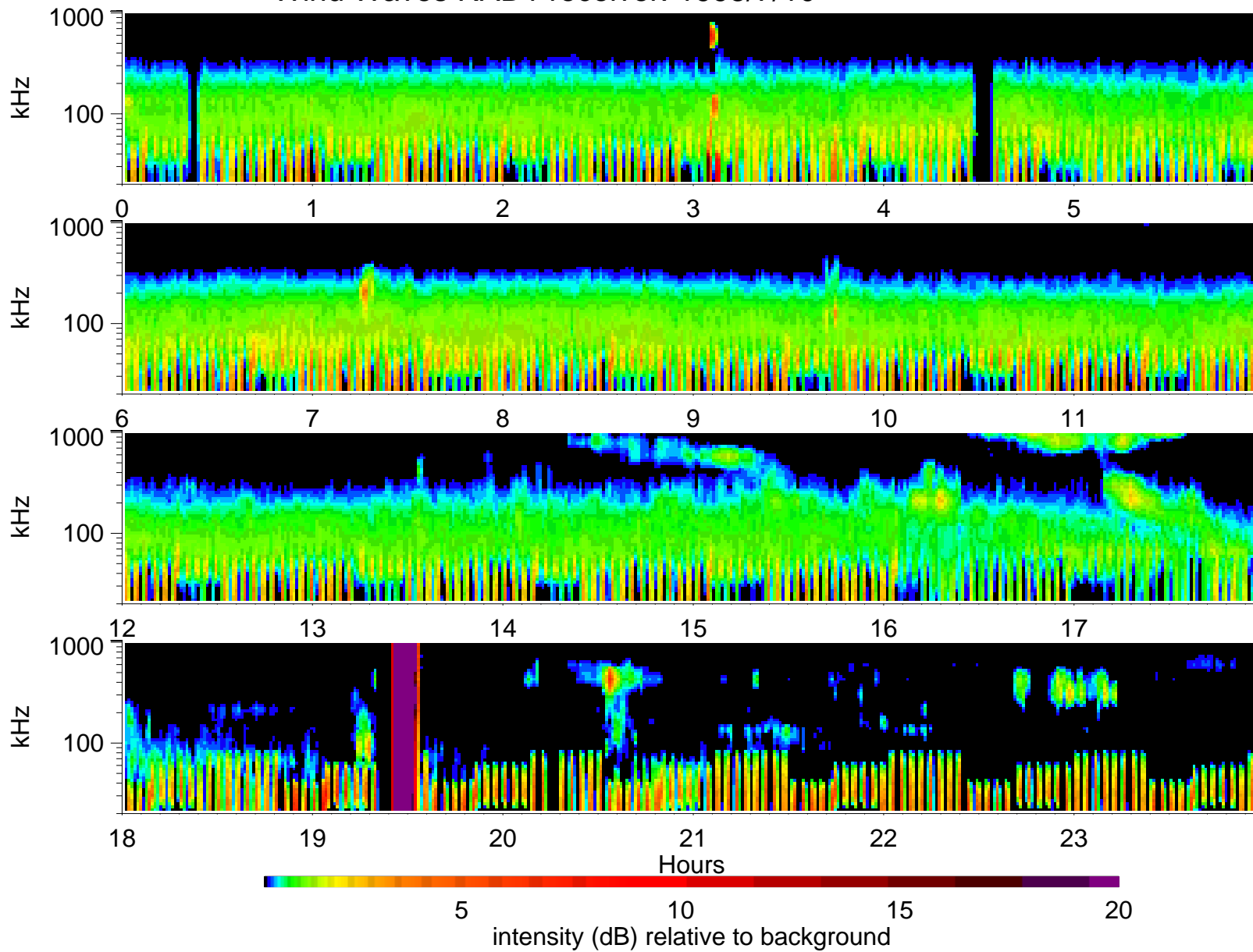
Wind Waves RAD1 receiver: 1995/7/10
