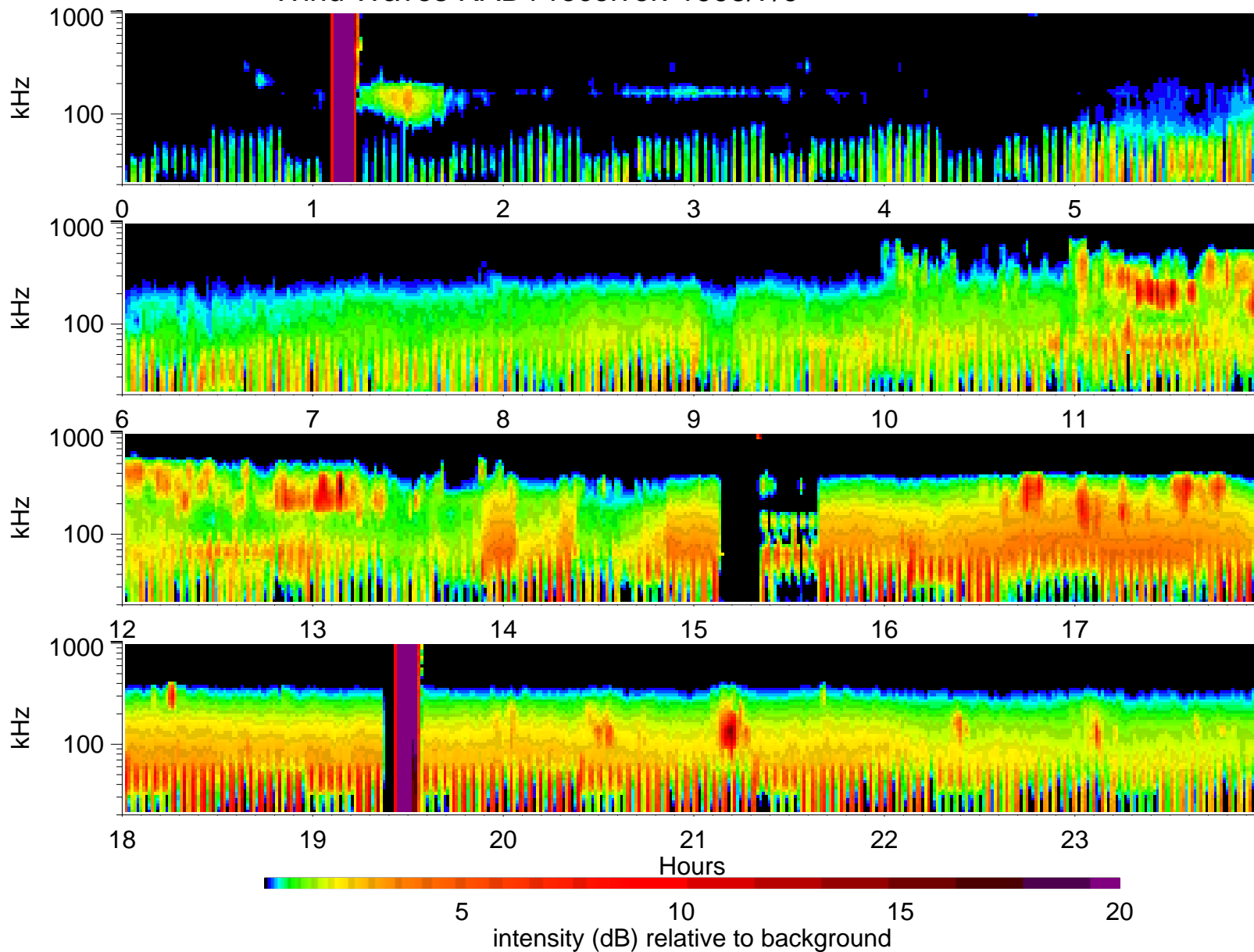
Wind Waves RAD1 receiver: 1995/7/9
