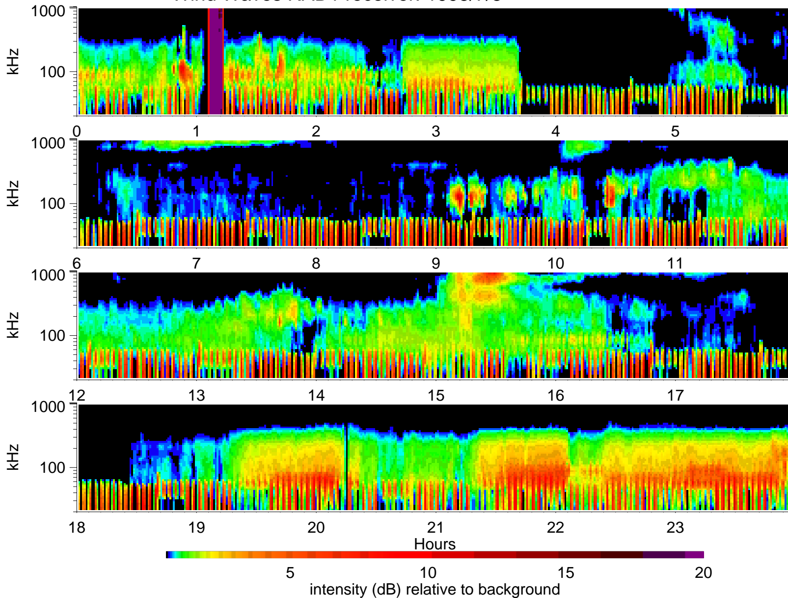
Wind Waves RAD1 receiver: 1995/7/3
