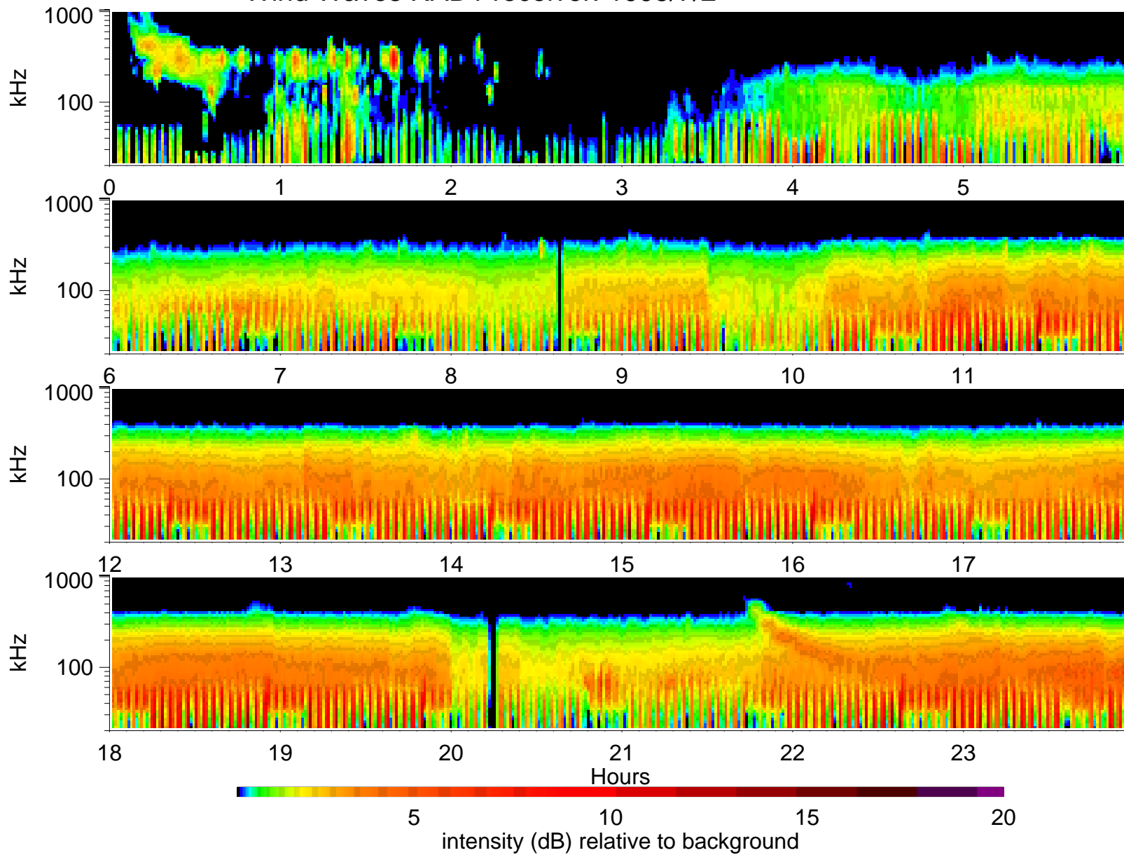
Wind Waves RAD1 receiver: 1995/7/2
