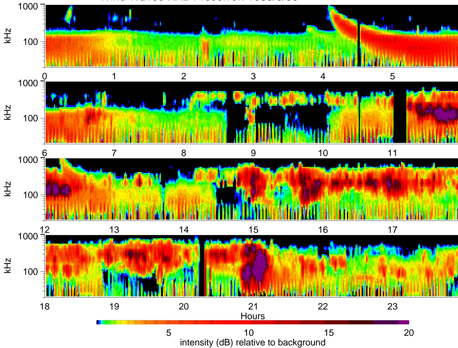
Wind Waves RAD1 receiver: 1995/6/30
