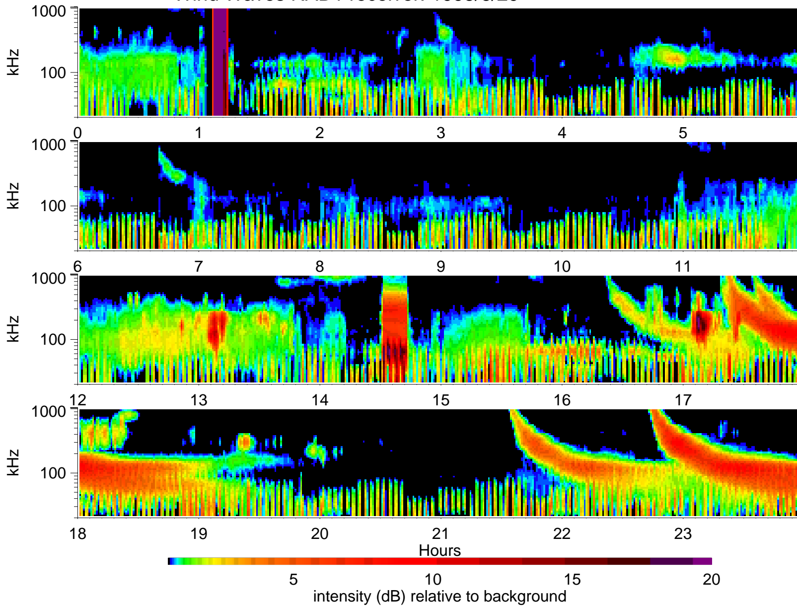
Wind Waves RAD1 receiver: 1995/6/29
