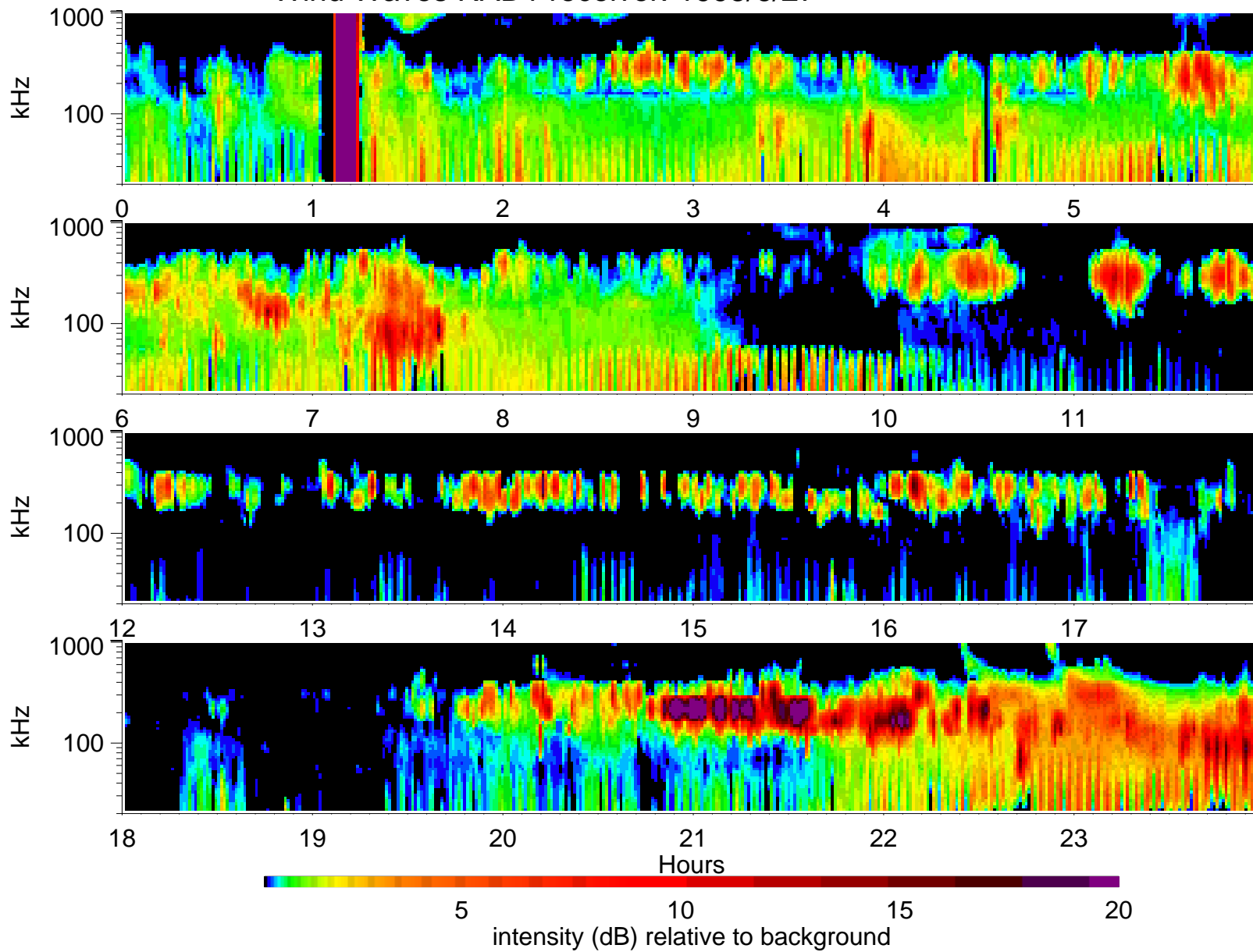
Wind Waves RAD1 receiver: 1995/6/27
