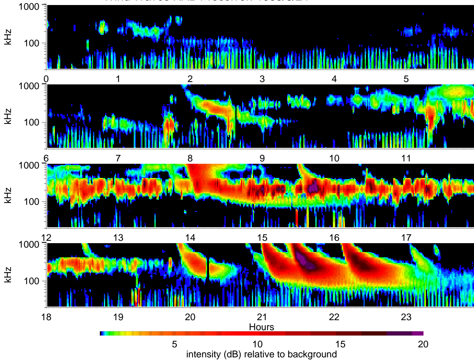
Wind Waves RAD1 receiver: 1995/6/24
