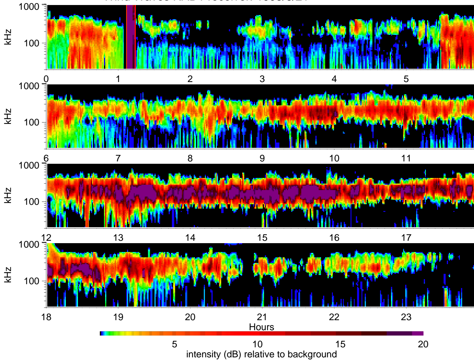
Wind Waves RAD1 receiver: 1995/6/21
