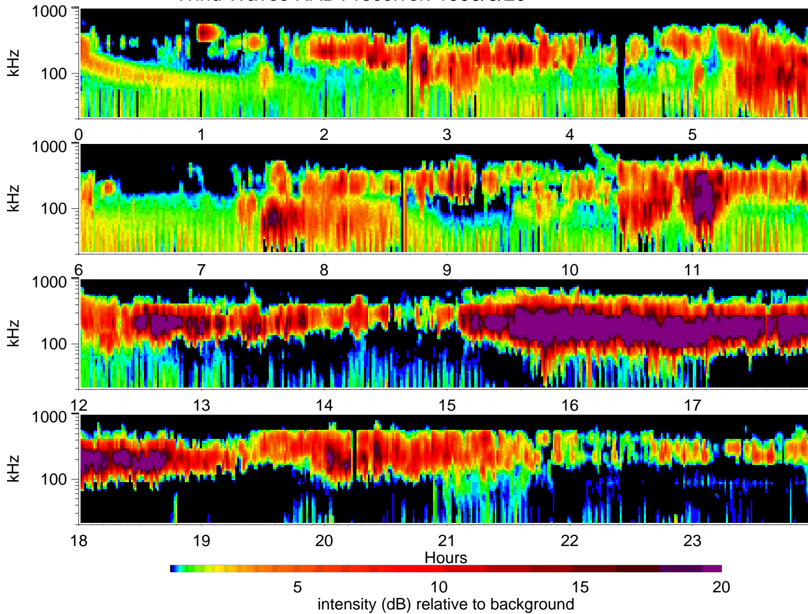
Wind Waves RAD1 receiver: 1995/6/20
