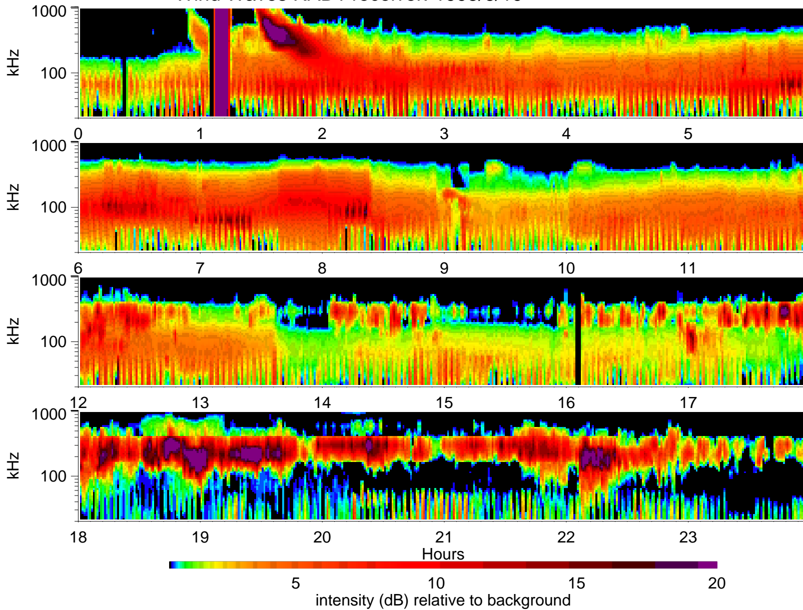
Wind Waves RAD1 receiver: 1995/6/19
