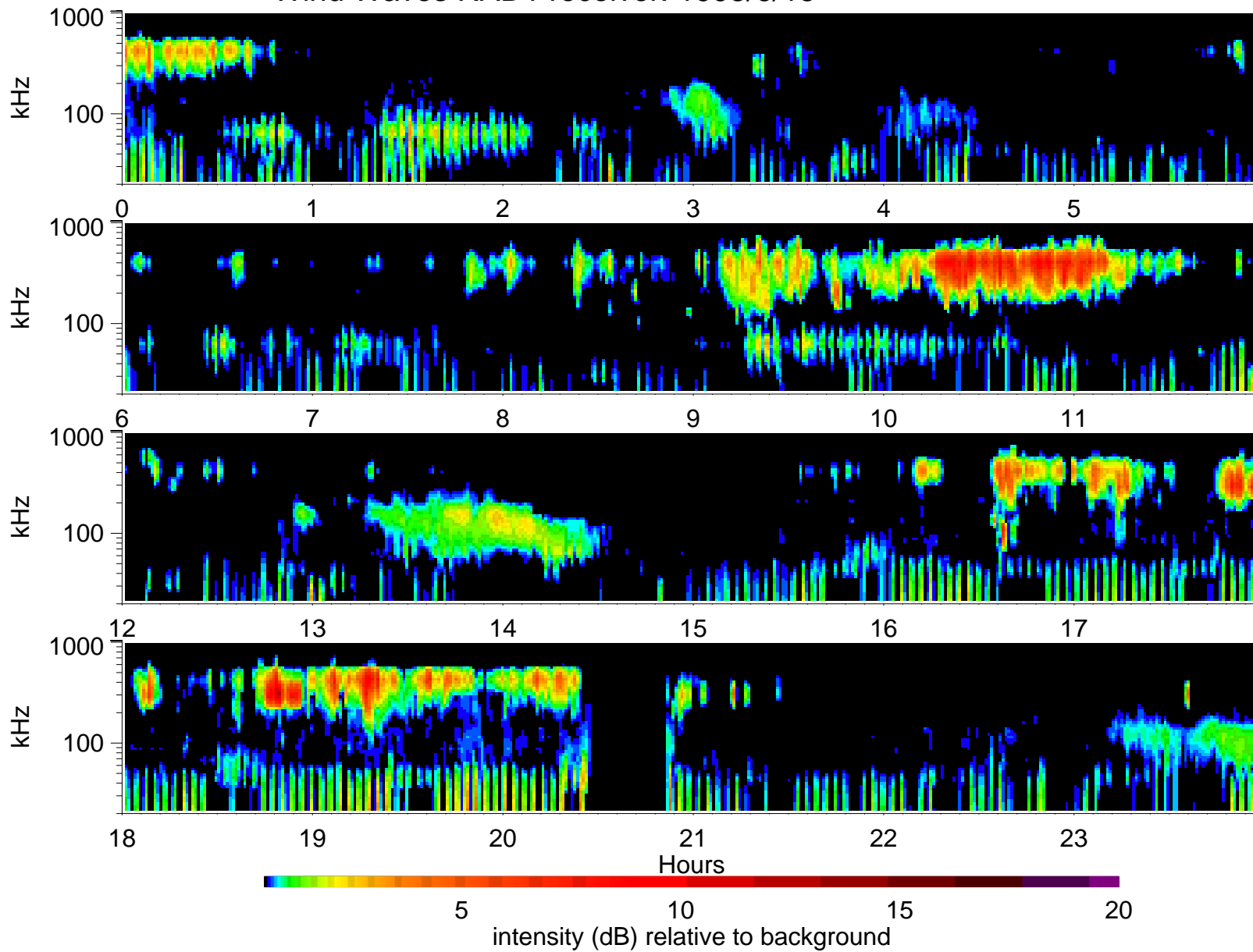
Wind Waves RAD1 receiver: 1995/6/15
