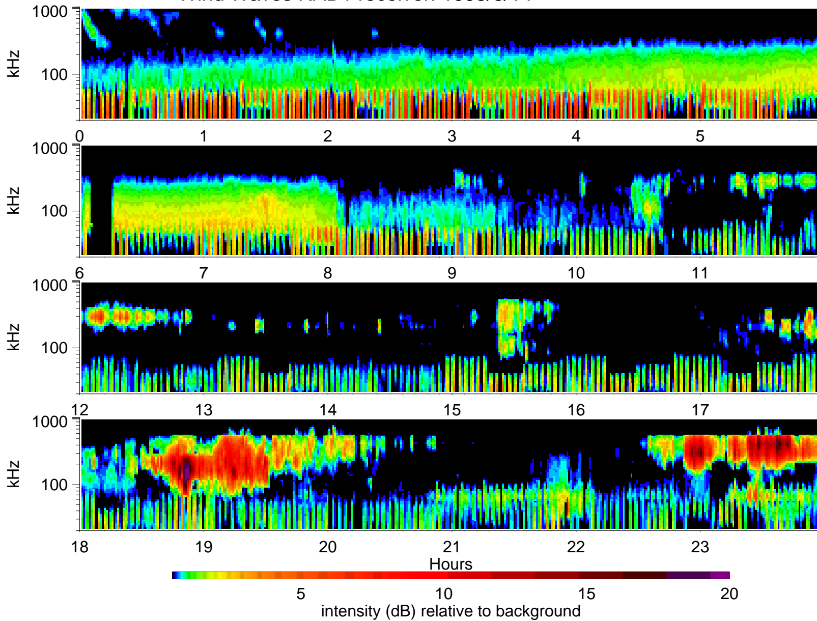
Wind Waves RAD1 receiver: 1995/6/14
