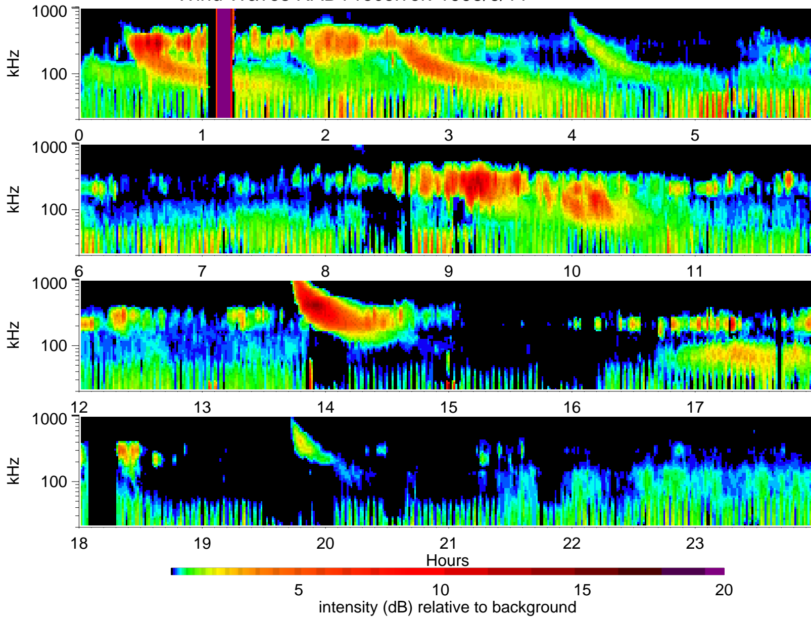
Wind Waves RAD1 receiver: 1995/6/11
