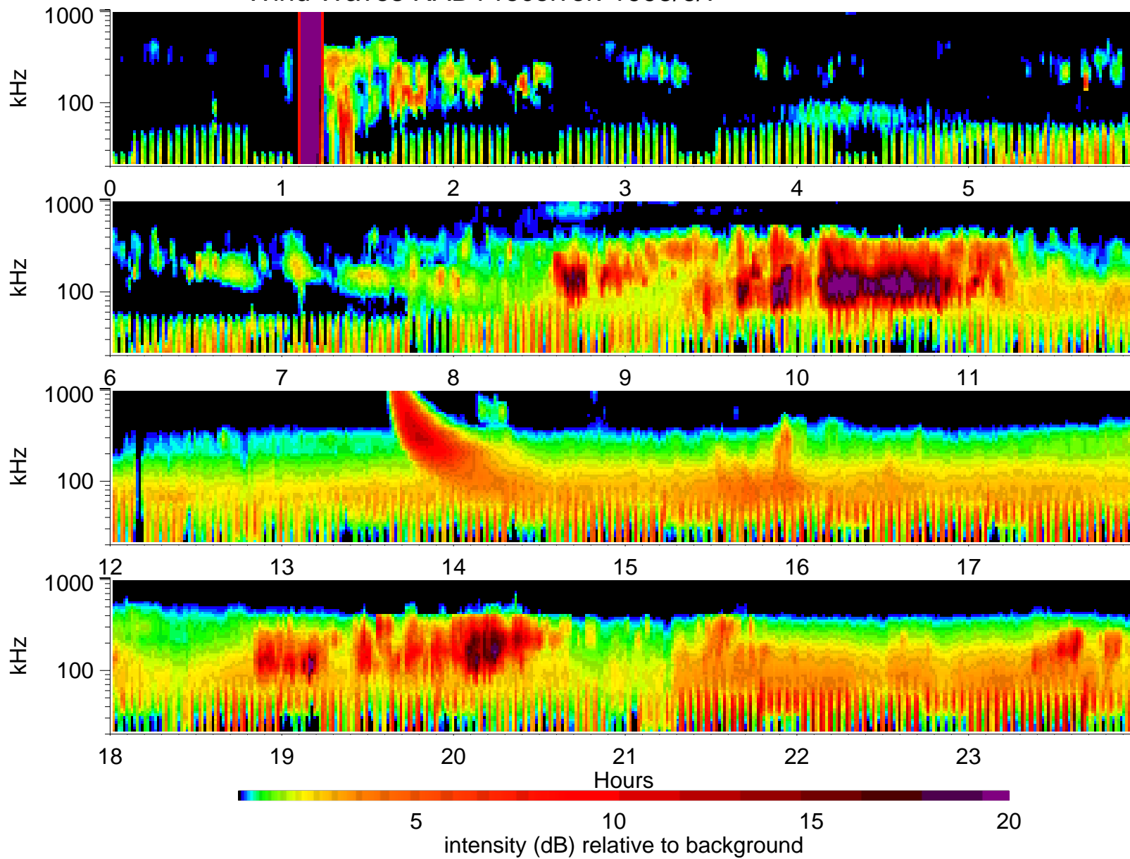
Wind Waves RAD1 receiver: 1995/6/7
