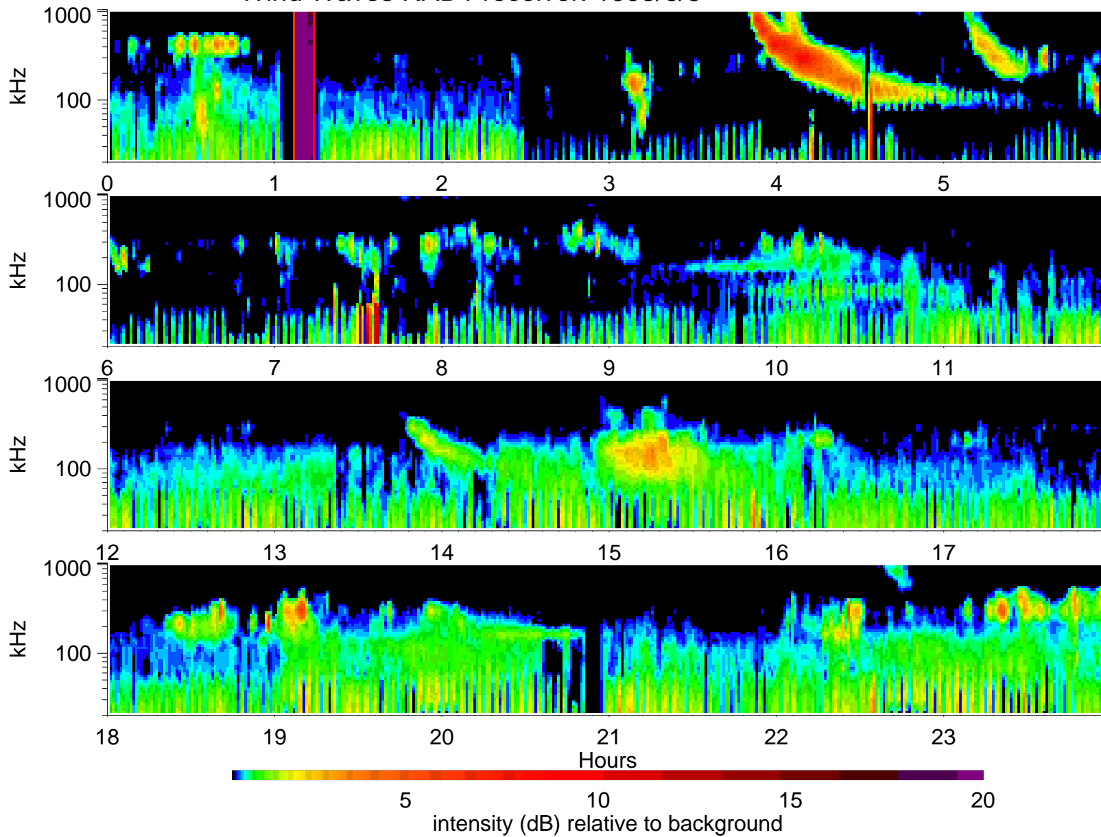
Wind Waves RAD1 receiver: 1995/6/5
