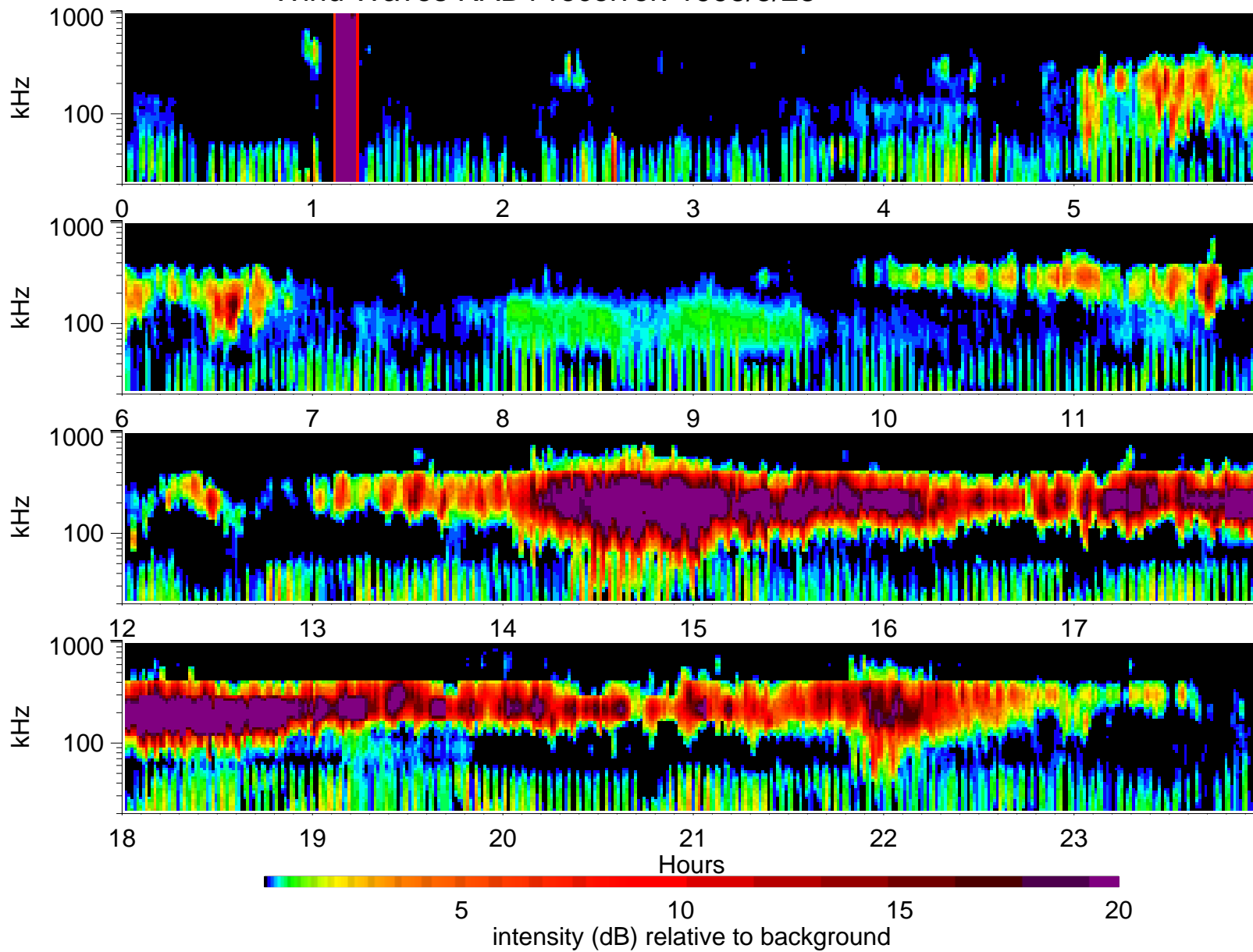
Wind Waves RAD1 receiver: 1995/5/28
