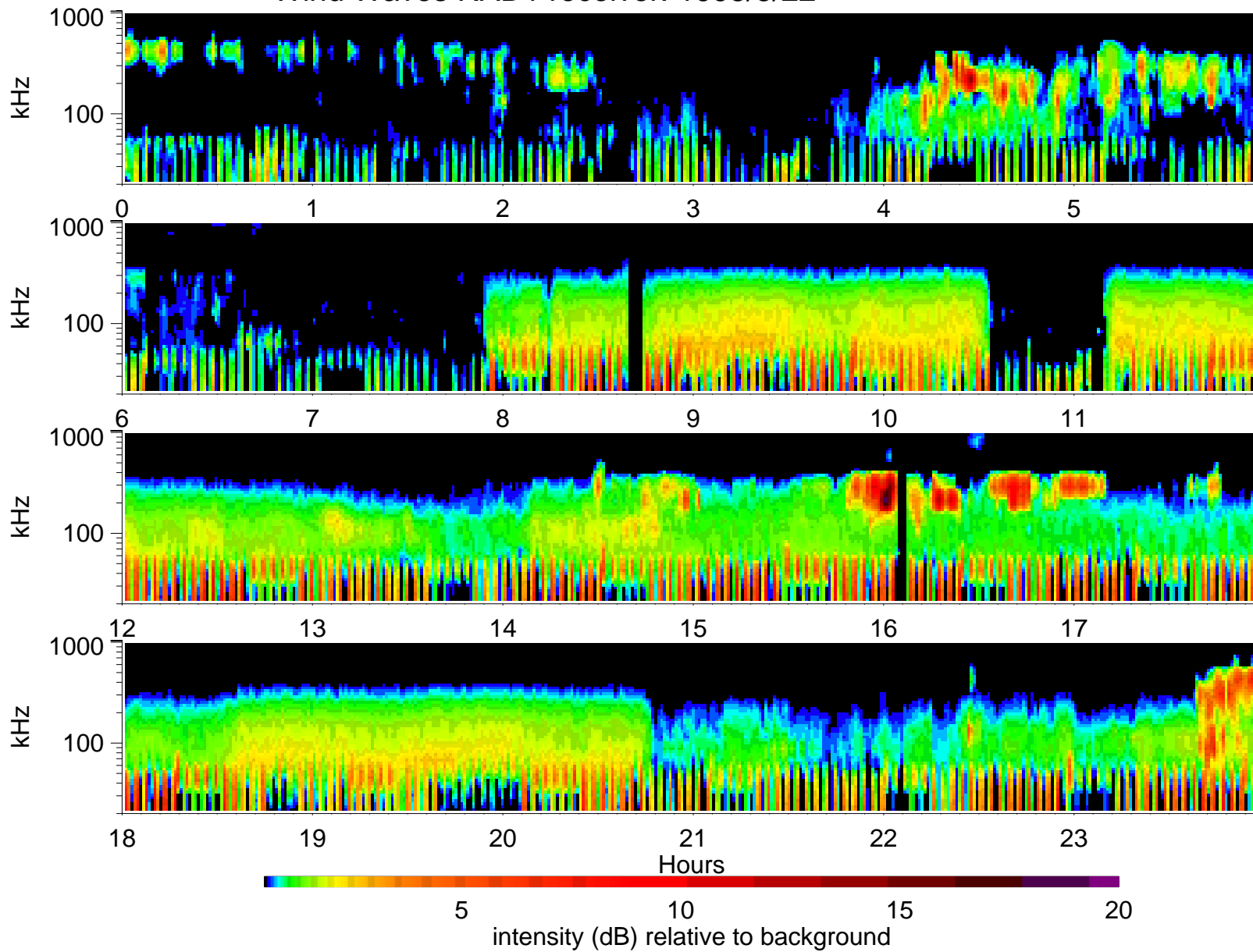
Wind Waves RAD1 receiver: 1995/5/22
