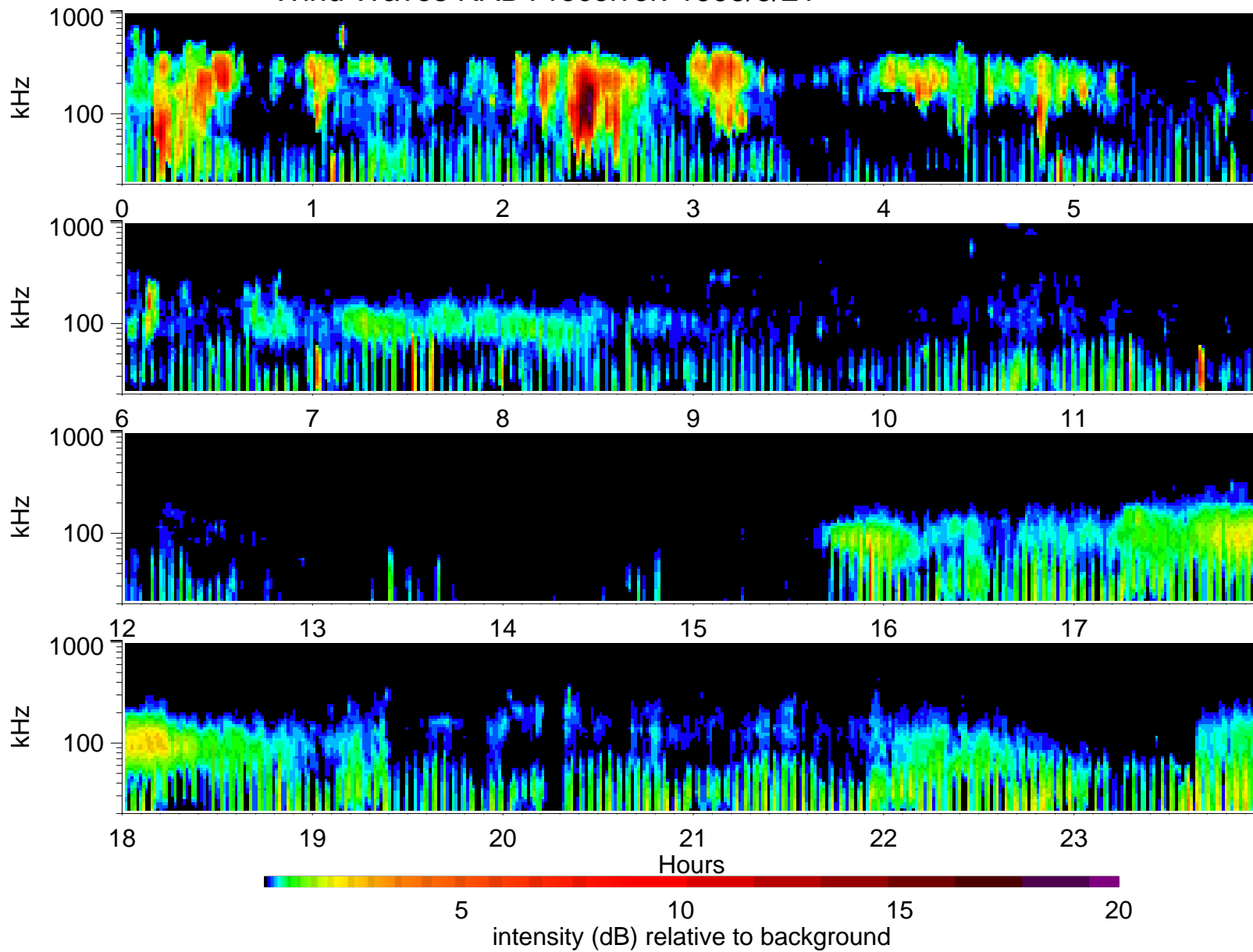
Wind Waves RAD1 receiver: 1995/5/21
