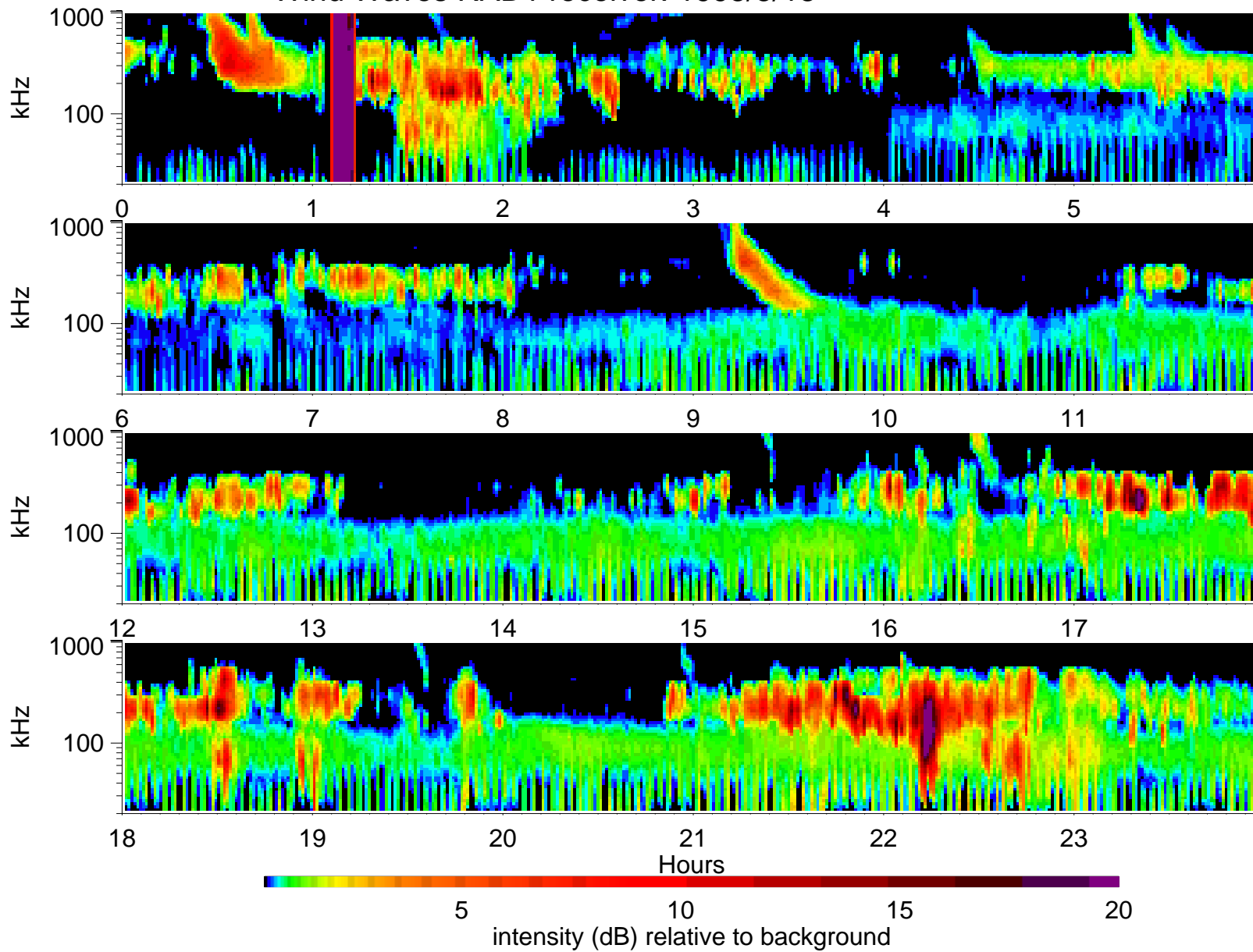
Wind Waves RAD1 receiver: 1995/5/18
