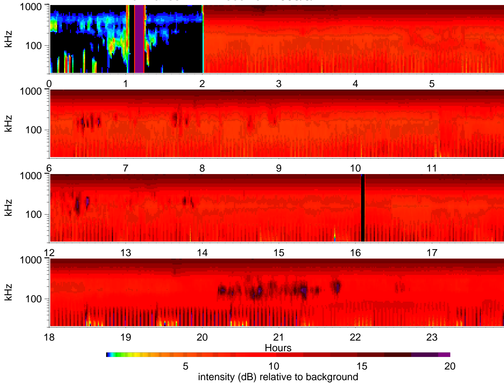
Wind Waves RAD1 receiver: 1995/5/12
