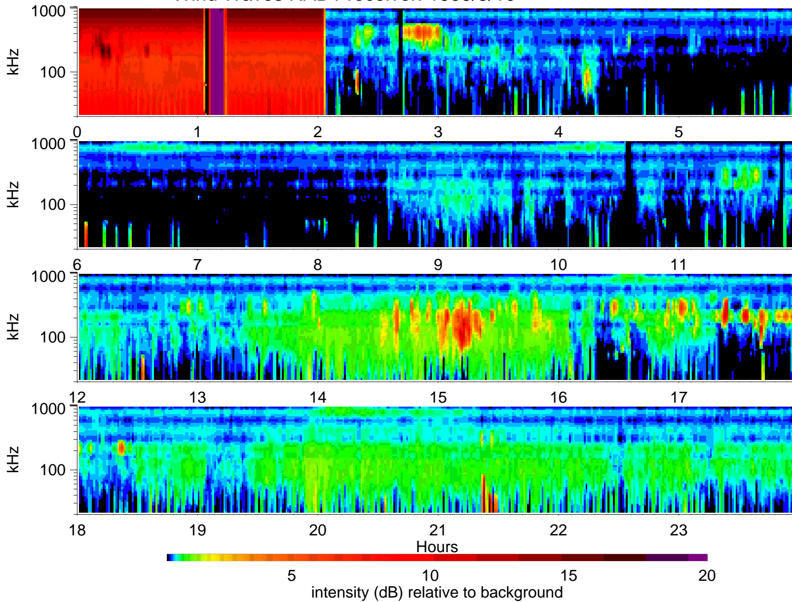
Wind Waves RAD1 receiver: 1995/5/10
