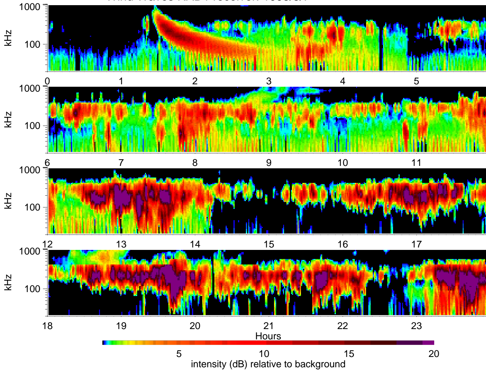
Wind Waves RAD1 receiver: 1995/5/7
