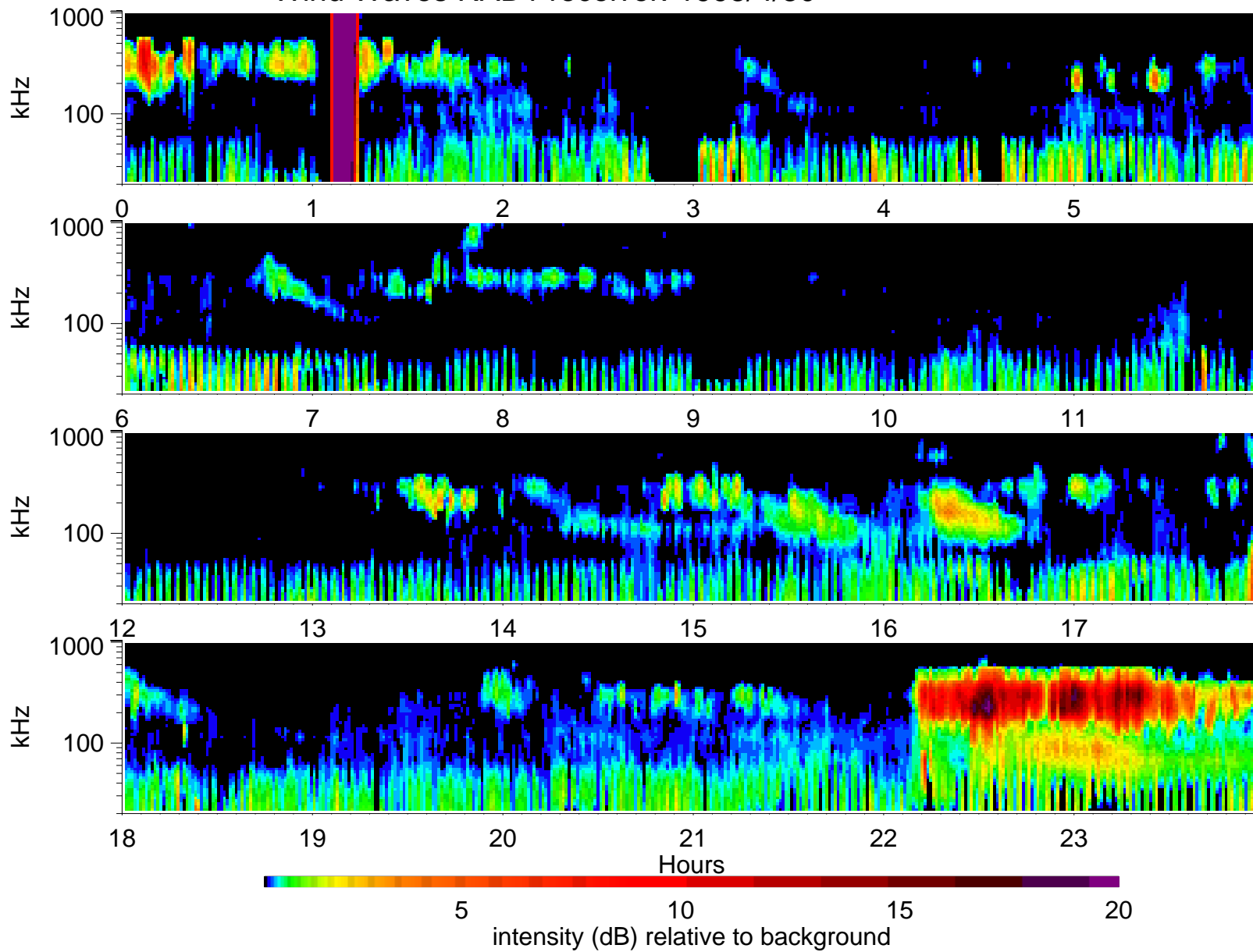
Wind Waves RAD1 receiver: 1995/4/30
