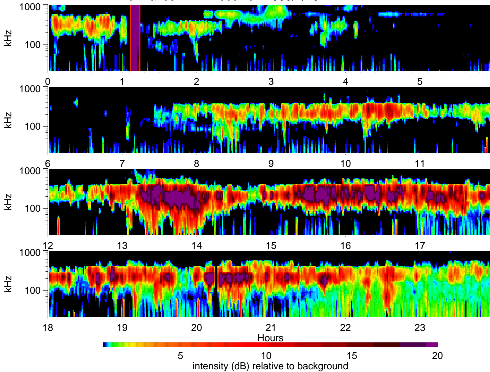
Wind Waves RAD1 receiver: 1995/4/29
